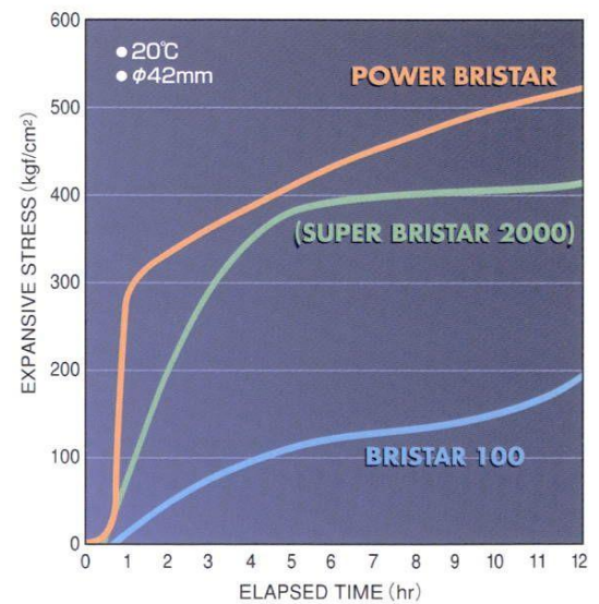
RELATIONSHIP OF EXPANSIVE STRESS AMONG POWER BRISTAR, SUPER BRISTAR 2000 AND BRISTAR
